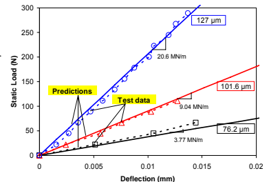
Fig. 8. Static force versus deflection for three bump strip layers with foil thickness 76.2 \mu\text{m} (3 mil), 101.6 \mu\text{m} (4 mil), and 127 \mu\text{m} (5 mil). Test data compared to model predictions using a dry-friction coefficient of 0.15
