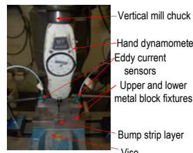
Fig. 7. Test rig for determining static stiffness of sample bump foils.
