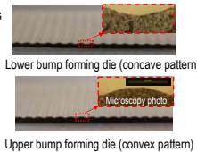
Fig. 3. Photographs of wire EDM upper and lower forming dies
