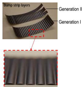
Fig. 5. Production of generation I and II bump strip layers
