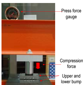
Fig. 4. Bump forming tools installed on hydraulic press machine
